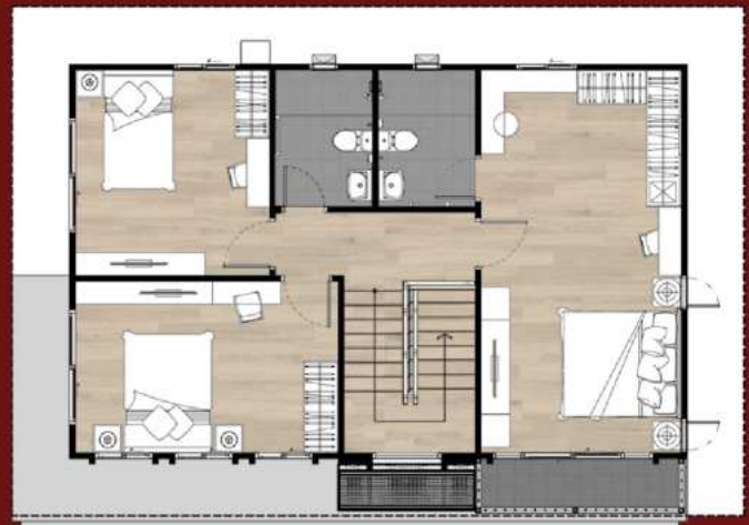
2ND FLOOR
